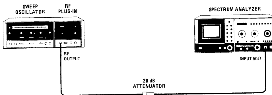
Figure 4-5. Residual FM Test Setup
