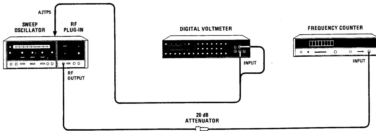
Figure 5-2. YIG Driver Frequency Adjustments Test Setup
