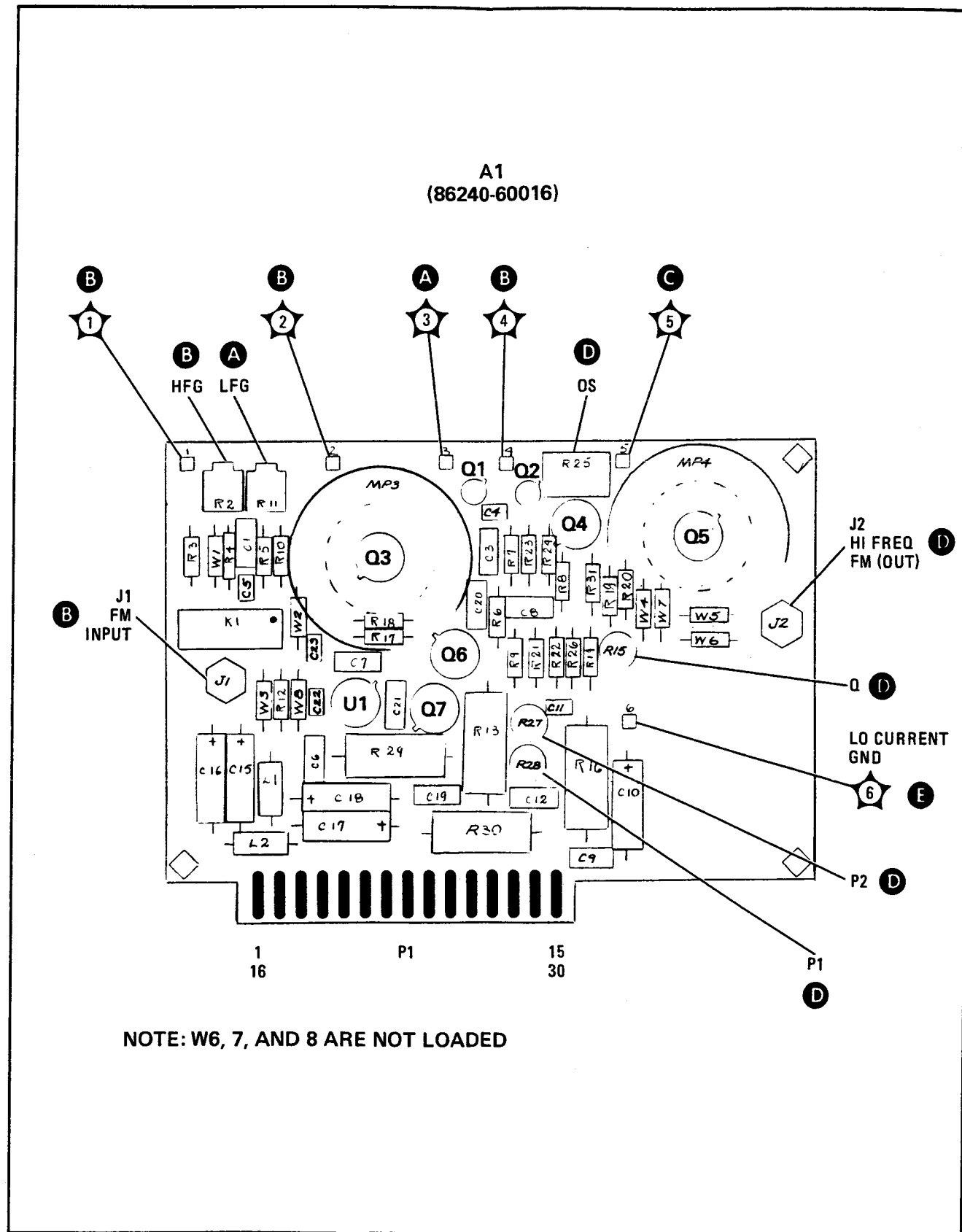
Figure 5-14. Test Point and Adjustment Locations for 86235A Option 008 and 86240C A1 FM Assembly
