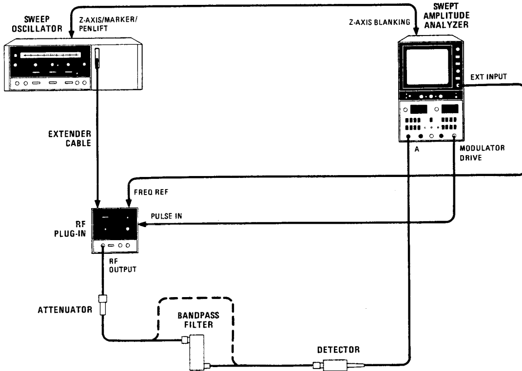
Figure 5-4. Harmonic Adjustments Test Setup
