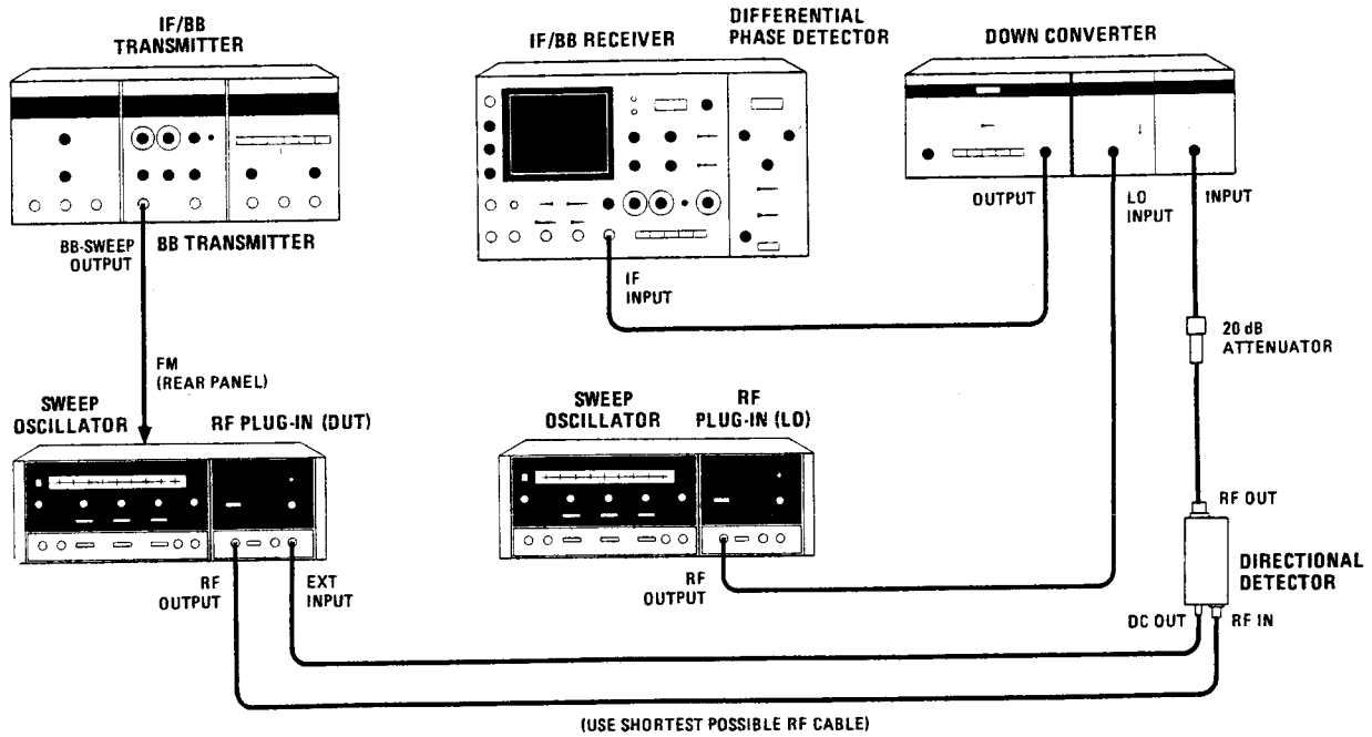
Figure 4-24. Up Converter Simulation Test Setup
