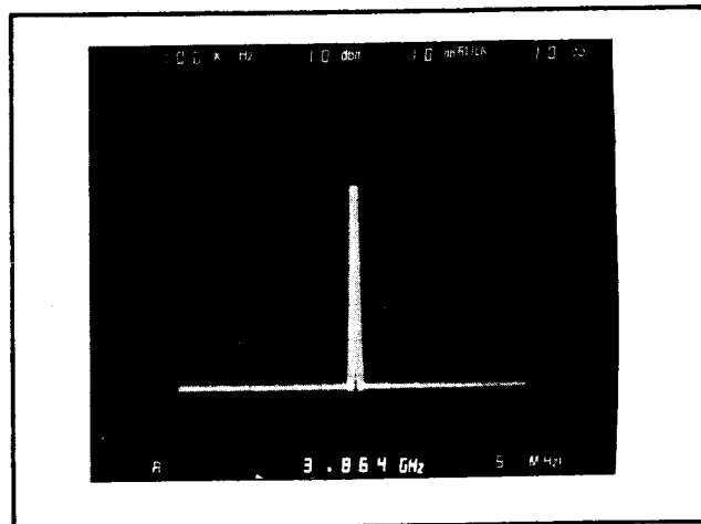
Figure 3-15. Spectrum Analyzer Display of Phase-Locked CW Signal
