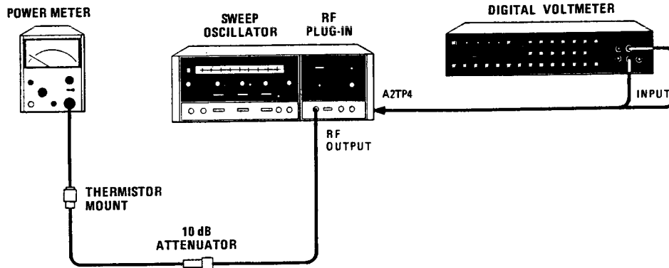
Figure 5-7. OFFSET and Power Control Adjustments Test Setup
