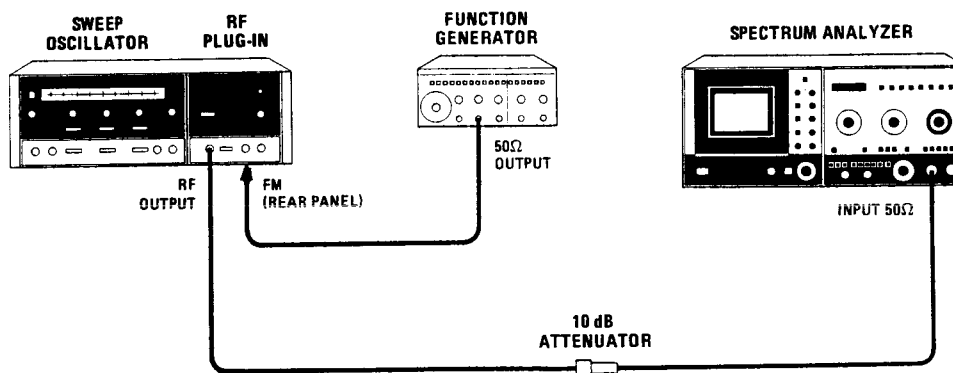
Figure 4-18. External FM Test Setup
