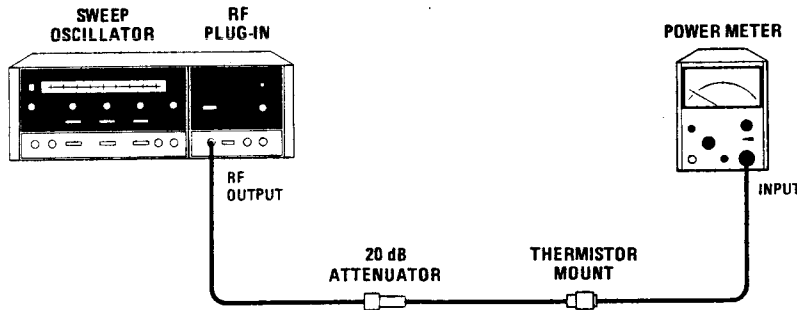
Figure 4-9. Internal Leveling Test Setup
