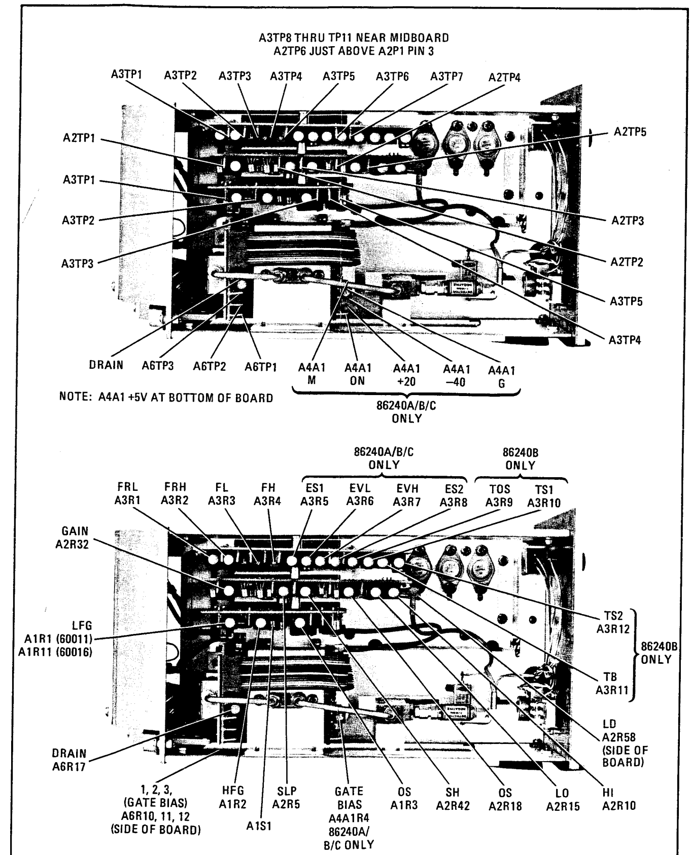
Figure 5-15. Test Point and Adjustment Locations
